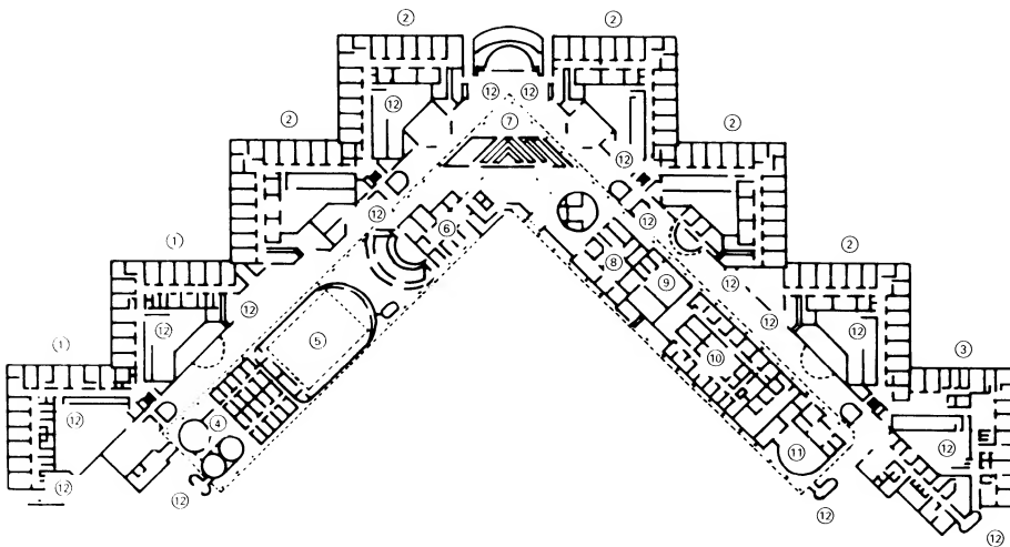
6 Capital District Psychiatric Center, Albany, New York accommodates 400 inpatients in 16 residential units, each of which serves 25 day patients
